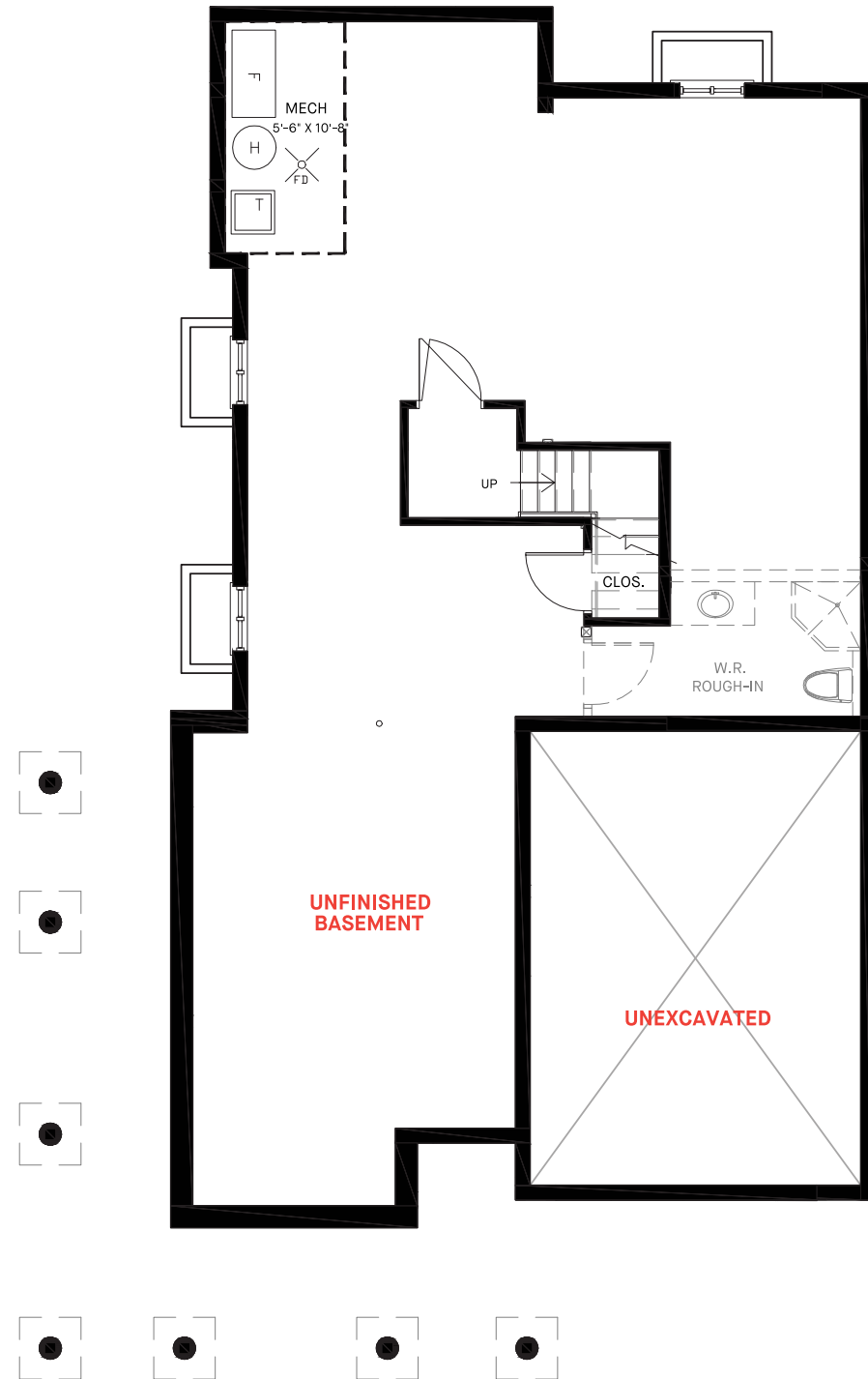
BASEMENT PLAN
